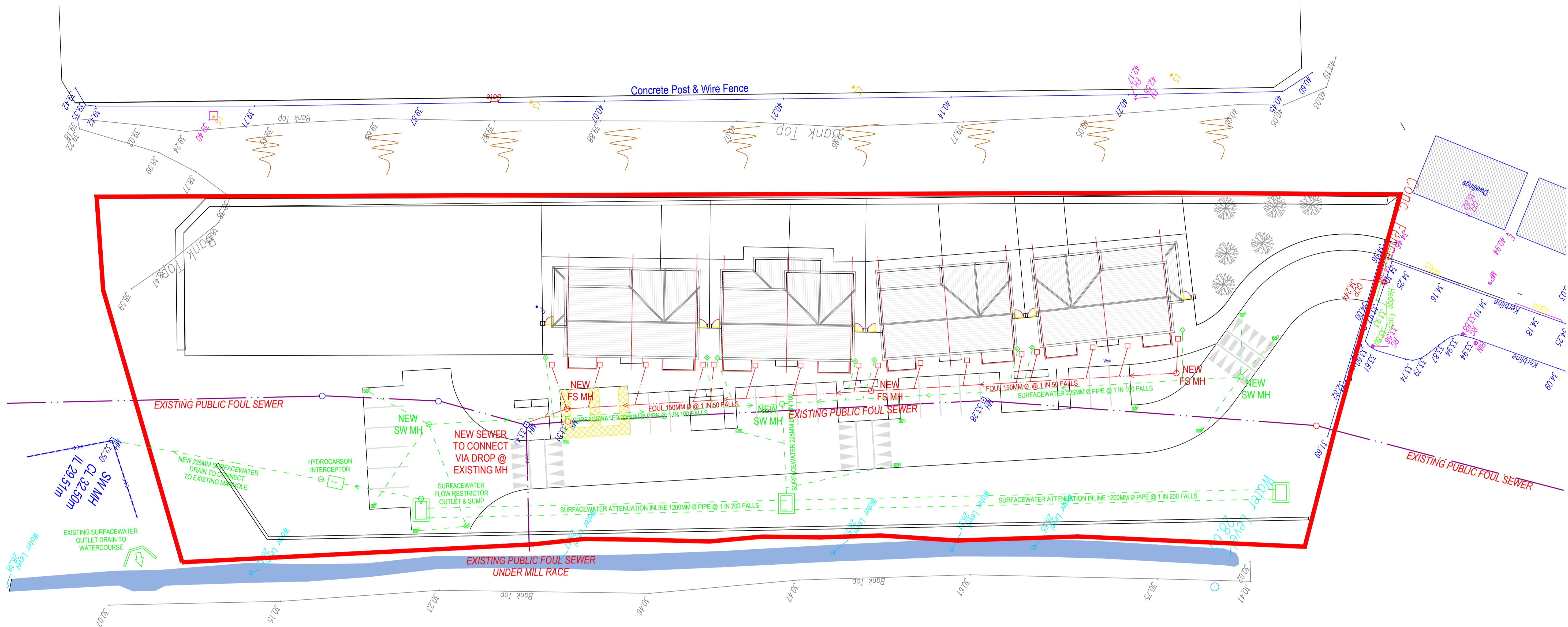
DRAINAGE LAYOUT SCALE 1:250
